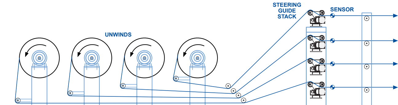
GUIDING FOUR WEBS ON A MULTI-WALL BAG MACHINE
