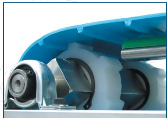
DualDrive with Volta supplied pulleys
